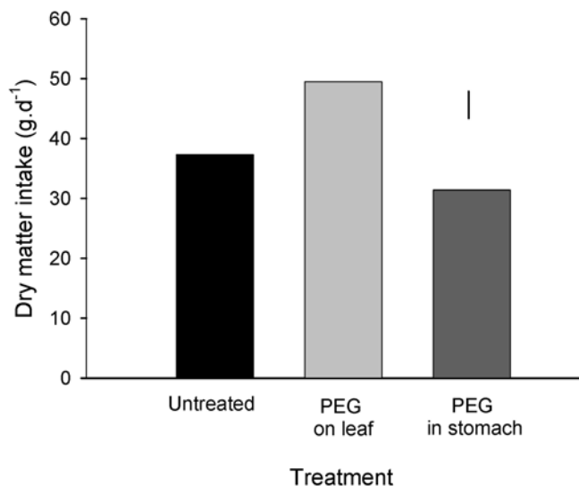
Fig. 7 The effect of PEG on the DMI by brushtail possums fed Eucalyptus melliodora foliage. The PEG was administered as a coating on the foliage or by gavage. The bar represents the 5% least significant difference. P_{\text{treatment}} < 0.001
