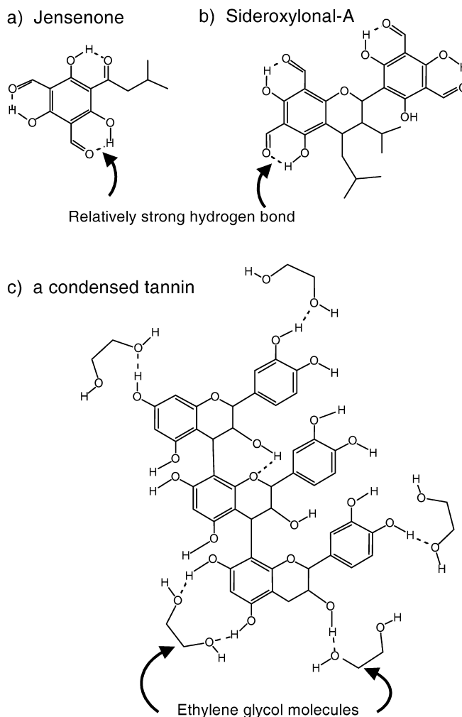
Fig. 1a–c The structures of the formylated phloroglucinol compounds (FPCs) jensenone (a) and sideroxydonal-A (b), and of a condensed tannin (c). FPCs show relatively strong intra-molecular hydrogen bonding (O–H) that prevents bonding by polyethylene glycol (PEG). Tannins have only weak potential for intra-molecular hydrogen bonding, and inter-molecular hydrogen bonding with PEG inactivates the tannin
